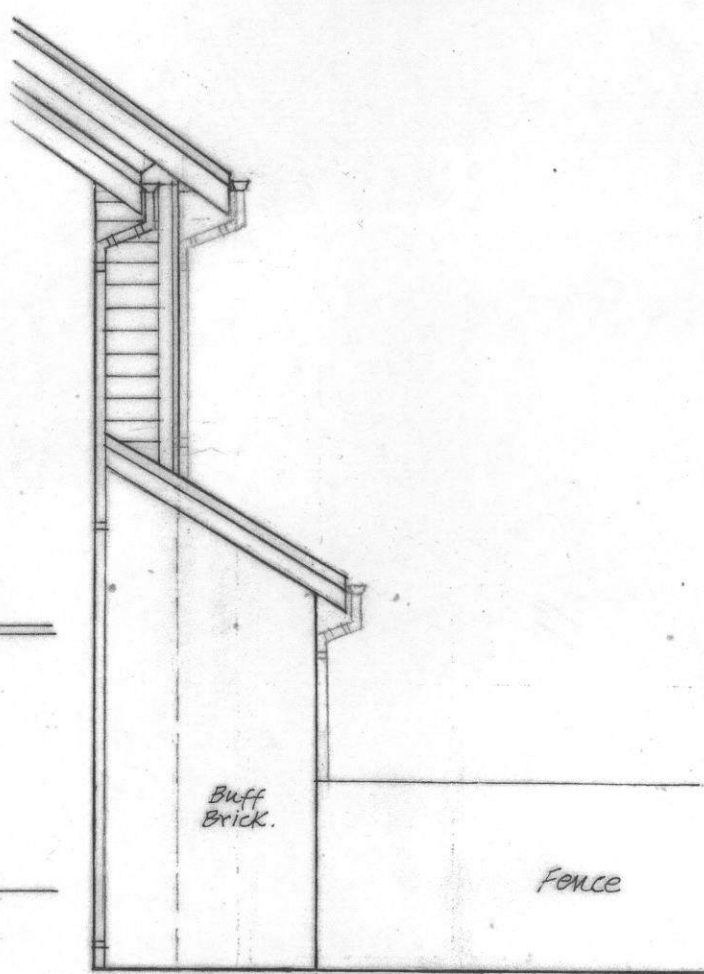
Existing Side View 1:50
